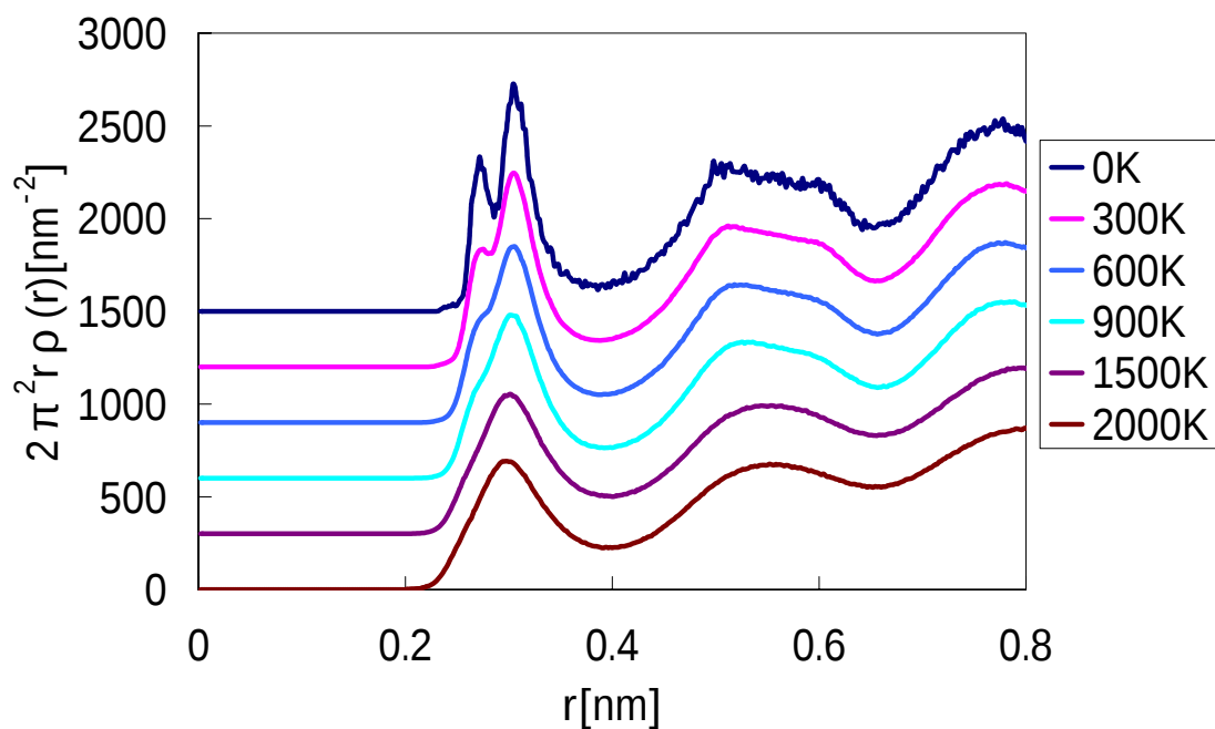
Fig 3.3.2 Radial distribution function of \text{Zr}_{70}\text{Ni}_{30} amorphous metals
