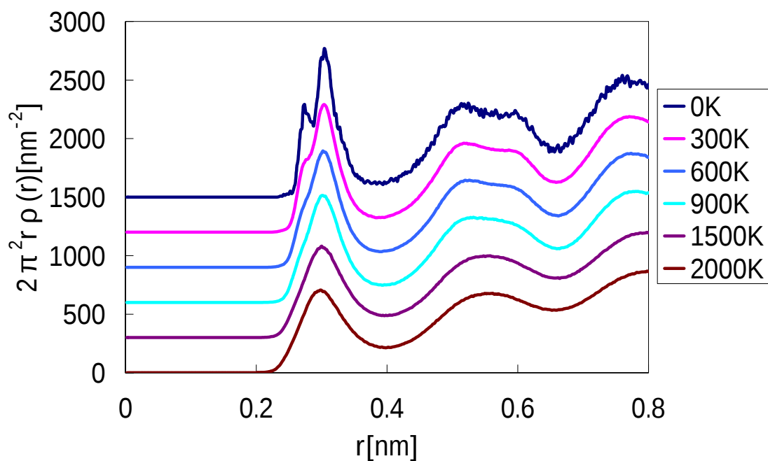
Fig 3.3.1 Radial distribution function of \text{Zr}_{70}\text{Cu}_{30} amorphous metals
