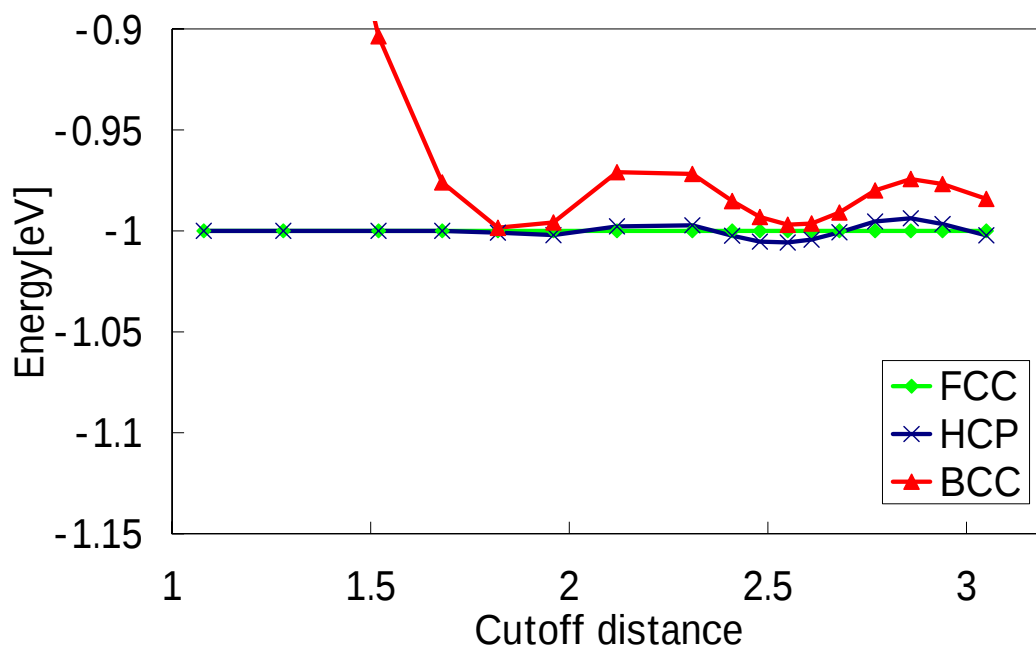
Fig 4.11.4 Cutoff distance vs. cohesive energy of each structure. ( D_c=0.5 )
