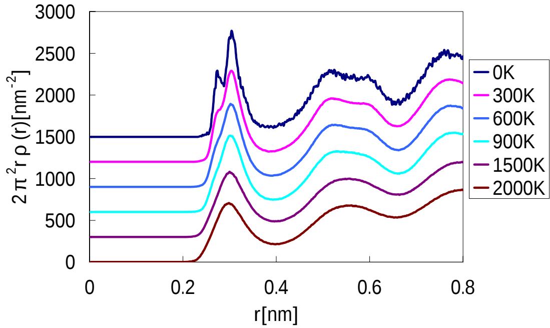
Fig 3.4.6 Radial distribution function of Zr 70 Ni 20 Al 10 metallic glass
