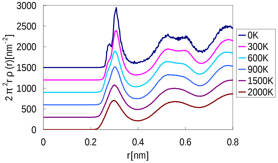
Fig 3.4.1 Radial distribution function of \text{Zr}_{70}\text{Cu}_{20}\text{Al}_{10} metallic glass
