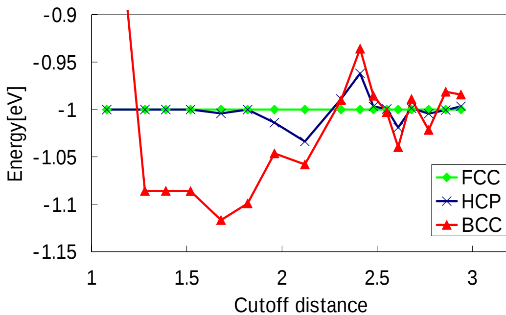
Fig 4.11.2 Cutoff distance vs. cohesive energy of each structure. ( D_c=0.1 )
