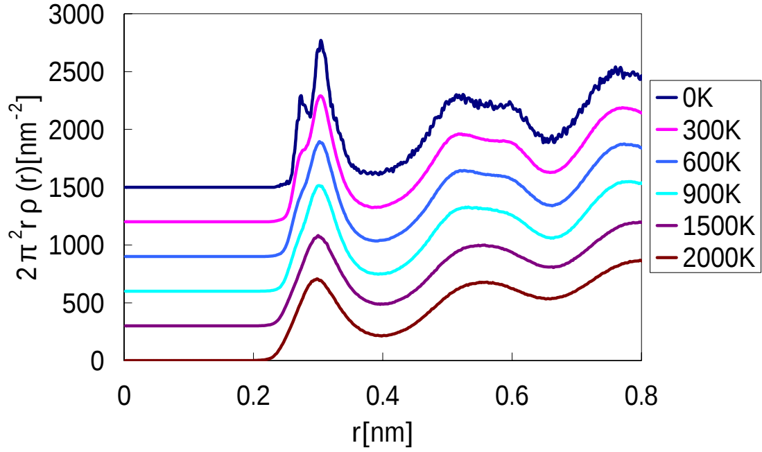
Fig 3.4.5 Radial distribution function of Zr 70 Cu 20 Al 10 metallic glass
