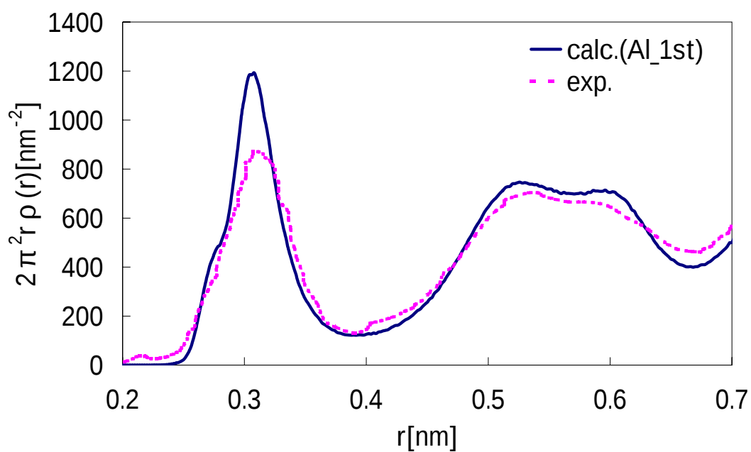
Fig 3.4.3 Radial distribution function of \text{Zr}_{70}\text{Cu}_{20}\text{Al}_{10} metallic glass
