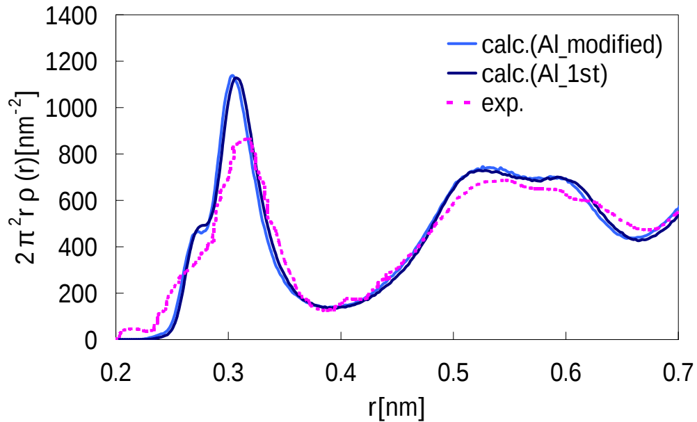
Fig 3.4.8 Radial distribution function of Zr_{70}Ni_{20}Al_{10} metallic glass
