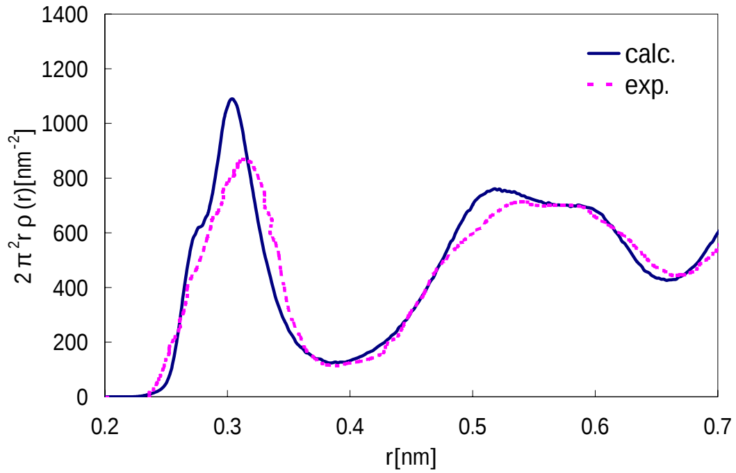
Fig 3.3.3 Radial distribution function of \text{Zr}_{70}\text{Cu}_{30} amorphous metals
