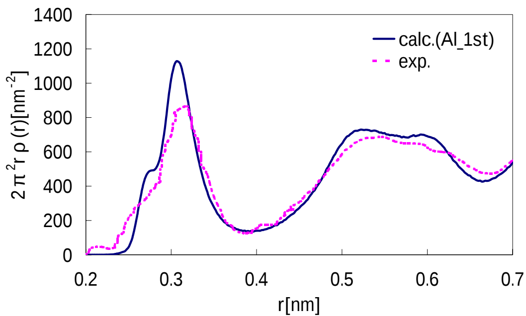
Fig 3.4.4 Radial distribution function of \text{Zr}_{70}\text{Ni}_{20}\text{Al}_{10} metallic glass
