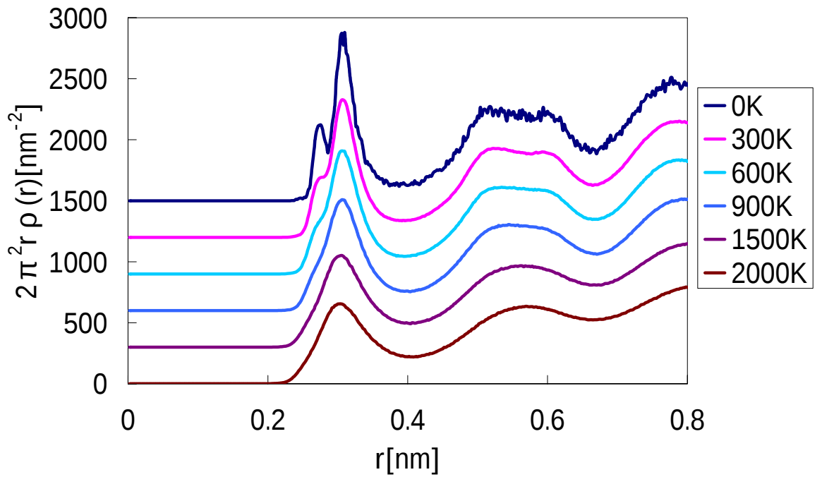
Fig 3.4.2 Radial distribution function of \text{Zr}_{70}\text{Ni}_{20}\text{Al}_{10} metallic glass
