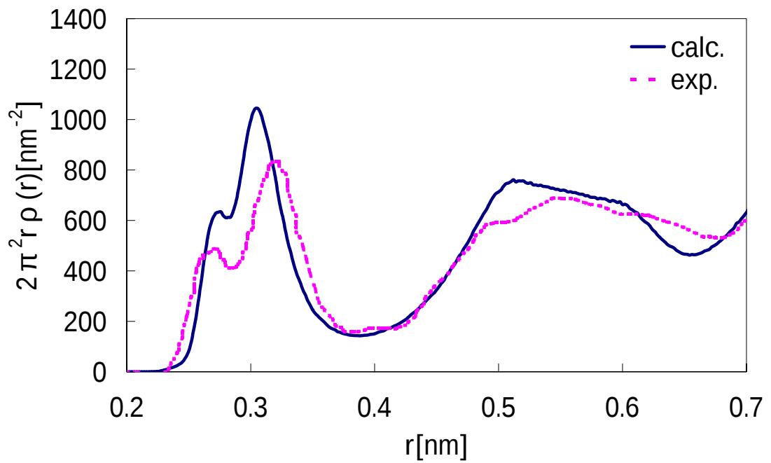
Fig 3.3.4 Radial distribution function of \text{Zr}_{70}\text{Ni}_{30} amorphous metals
